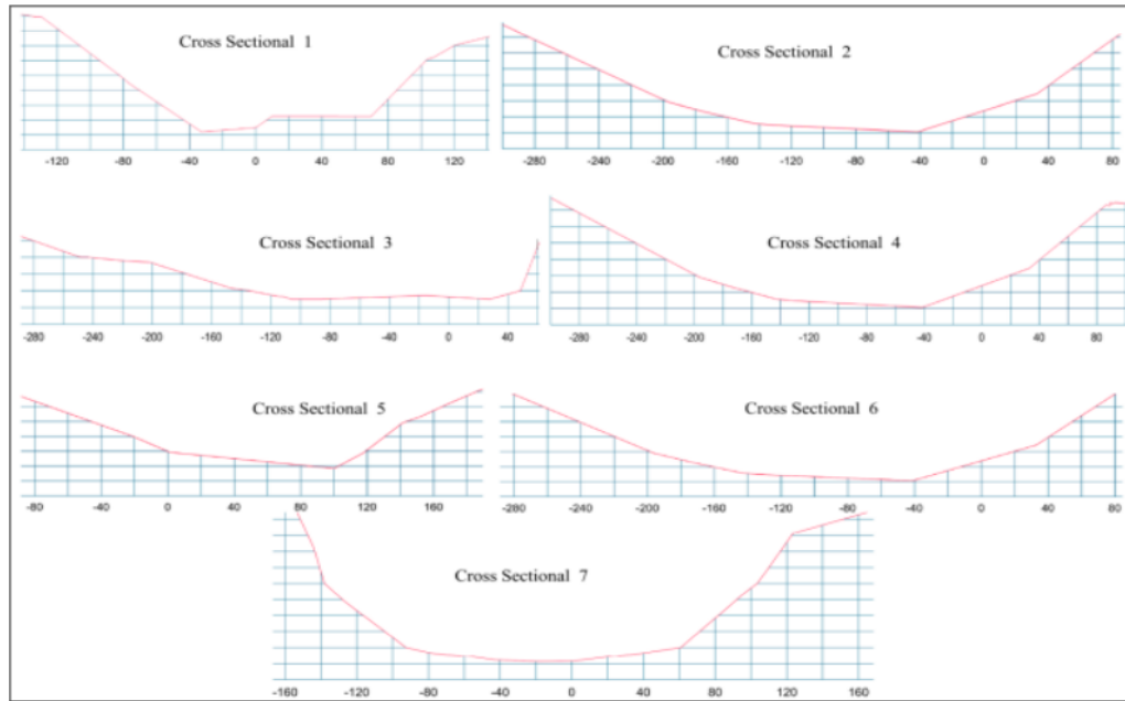
Figure5: Cross section, based on topographic survey 2014
