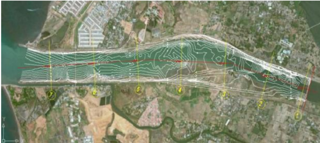
Figure3: Plan form and topographic contour, survey December 2014
